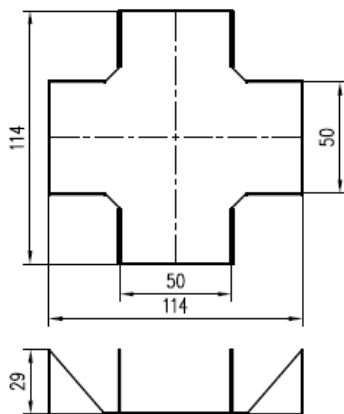
CROSS CONNECTOR TYPE A
