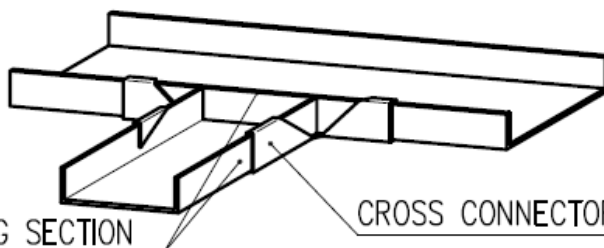
CROSS CONNECTOR TYPE A
