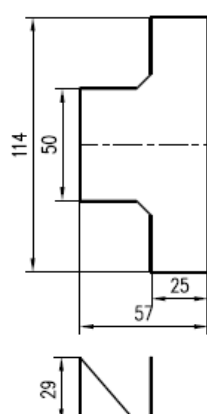
CROSS CONNECTOR TYPE B
